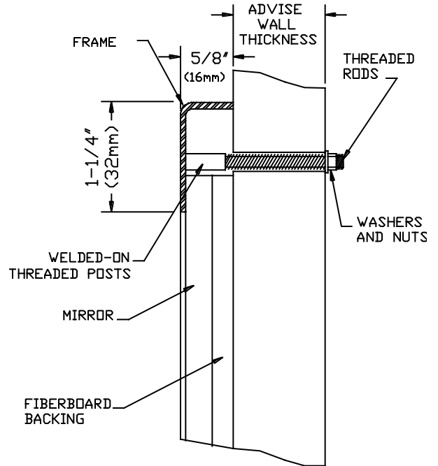
PARTIAL SECTION
