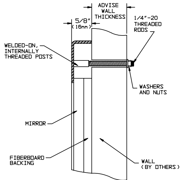
INSTALLATION DETAIL
